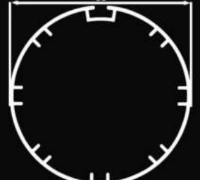
CODE: 34226 65 MM ALÜMİNYUM BORU
