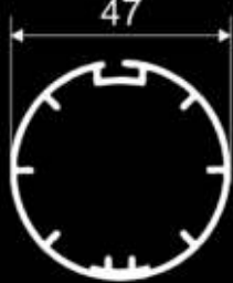
CODE: 34473 47 MM ALÜMİNYUM BORU
