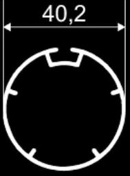
CODE: 34308 38 MM ALÜMİNYUM BORU
